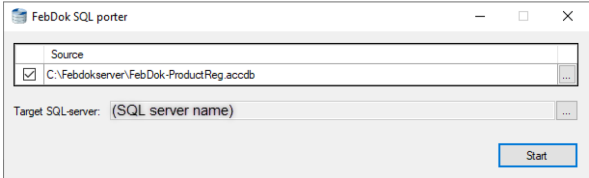
Figure 1 Click "Start".
